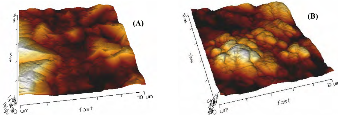
Fig. 7. AFM of pure nickel surface 3D – Heigh ( i = 4 \text{ A/dm}^2 for 1h ): (A) - untreated; (B)- with SRB bacteria
