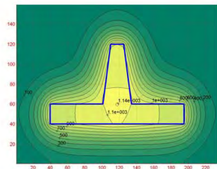
Fig. 14. Distribution of isotherms at the end of solidification for a rib of inclination \text{tg } \alpha = 9/60 and thickness b_n = 15 \text{ mm} (at the moment of solidification t_{\text{sol}} = 490.94\text{s} ).
