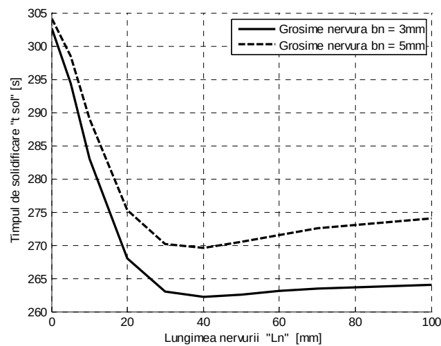
Fig. 15. Influence of rib length " L_n " on the solidification time for a cast iron plate of thickness a = 20\text{ mm} ( b_n = rib thickness; L_n = rib length).
