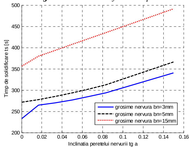
Fig. 16. The influence of rib inclination ( \tan \alpha ) on solidification time (part thickness a = 20\text{mm} , inclinations by increasing rib wall thickness) ( t_s = solidification time, \tan \alpha = rib wall inclination, b_n = rib thickness).
