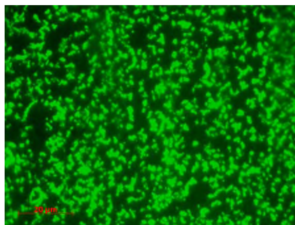
Fig. 3. Fluorescence microscopy image of SRB on pure nickel surface obtained at current density 4A/dm 2 , 60min.
