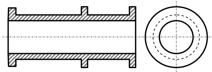
Fig. 1. Example of a part with thermal knot.
