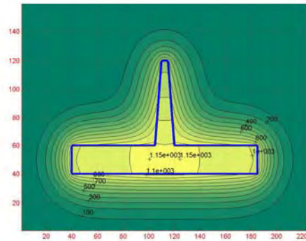
Fig. 9. Distribution of isotherms at the end of solidification for a rib of inclination \text{tg } \alpha = 5/60 and thickness b_n = 5 \text{ mm} (at the moment of solidification t_{\text{sol}} = 312.64\text{s} ).
