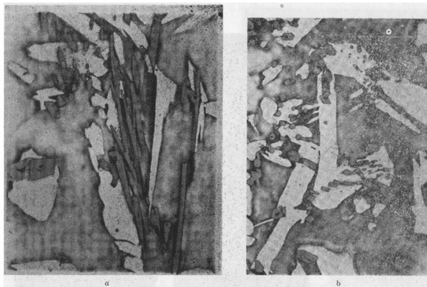
Fig. 4. a, b Morphology and distribution of the Mn_5Si_3 compound in the cast material. The needle-shaped compound Mn Si_3 (grey) is distributed in the solid solution \alpha (light colored) as well as in the solid solution (dark). Attack; FeCl_3 , ( \times 1000 ).
