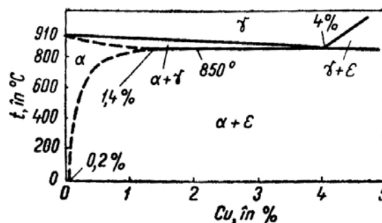
Fig. 6. Diagram of the Fe-Cu binary system.
