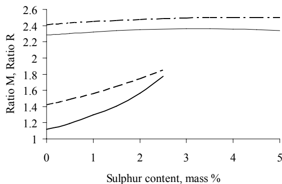
Fig. 4. Evolution of the ratio R=\sigma_i/\sigma and of the ratio M=\partial\sigma_i/\partial(S) / \partial\sigma/\partial(S) upon the sulphur content in slag \text{CaO-Al}_2\text{O}_3\text{-CaS} at 1873K; \sigma - surface tension in slag, \sigma_i -interfacial tension steel- slag, \partial\sigma_i/\partial(S) -concentration coefficient of the interfacial tension, \partial\sigma/\partial(S) - concentration coefficient of the surface tension.
