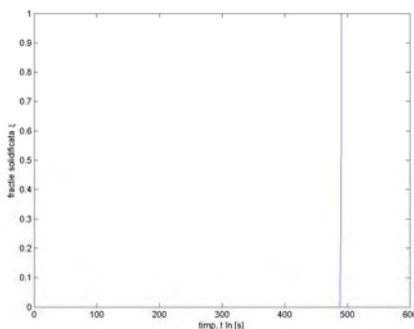
Fig. 20. Variation of the solid fraction in the hot spot (coordinates x = 0 mm, y = 9.5 mm), part with a rib of b_n = 15 mm and inclination \text{tg } \alpha = 9/60 . ( \xi = solid fraction).
