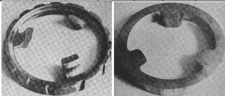
Fig. 1. Synchronous rings and mobile cone
