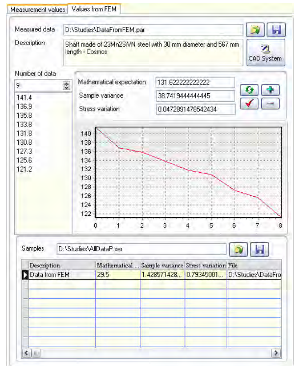
Fig. 6. Data obtained during measurements from testing of reducer shaft (a) and data obtained by the finite-element model (b).
