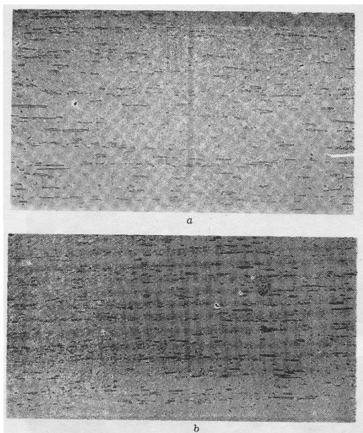
Fig. 4. a, b Morphology and distribution of the Mn_5Si_3 compound in the cast material. The needle-shaped compound Mn Si_3 (grey) is distributed in the solid solution \alpha (light colored) as well as in the solid solution (dark). Attack; FeCl_3 , ( \times 1000 ).
