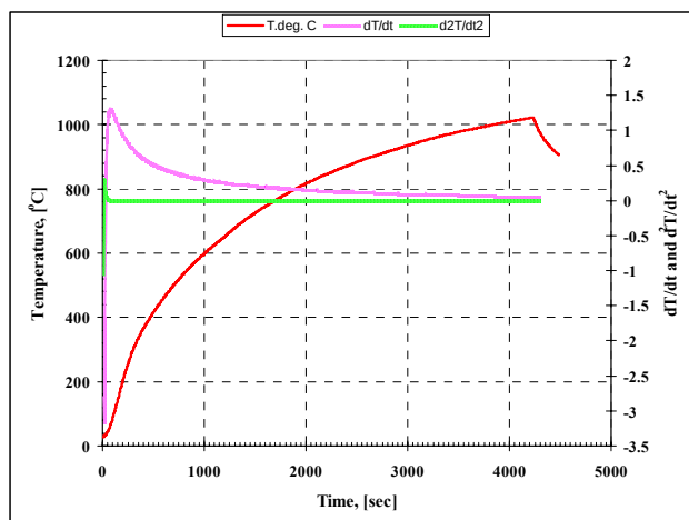
Fig. 3. Temperature-time dependencies used for tuning of the COMECO-RT1800 PID controller.
