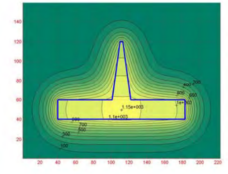
Fig. 6. Distribution of isotherms at the end of solidification for a rib of inclination \text{tg } \alpha = 9/60 and thickness b_n = 3 mm (at the moment of solidification t_{\text{sol}}=340.36\text{s} ).
