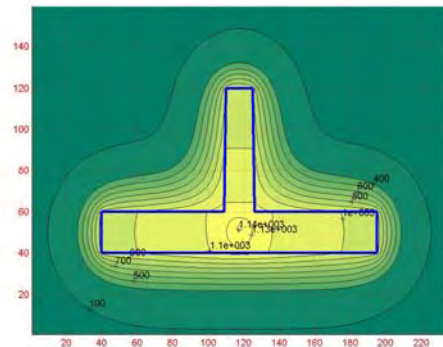
Fig. 11. Distribution of isotherms at the end of solidification for a rib of inclination \text{tg } \alpha = 1/60 and thickness b_n = 15 \text{ mm} (at the moment of solidification t_{\text{sol}} = 379.58\text{s} ).
