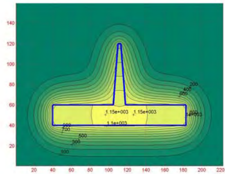
Fig. 5. Distribution of isotherms at the end of solidification for a rib of inclination \text{tg } \alpha = 5/60 and thickness b_n = 3 mm (at the moment of solidification t_{\text{sol}}=293.92\text{s} ).
