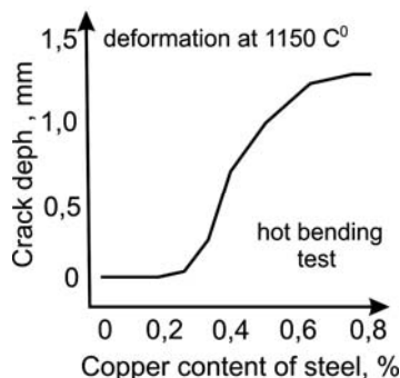
Fig. 5. Relation between copper content and crack depth.
