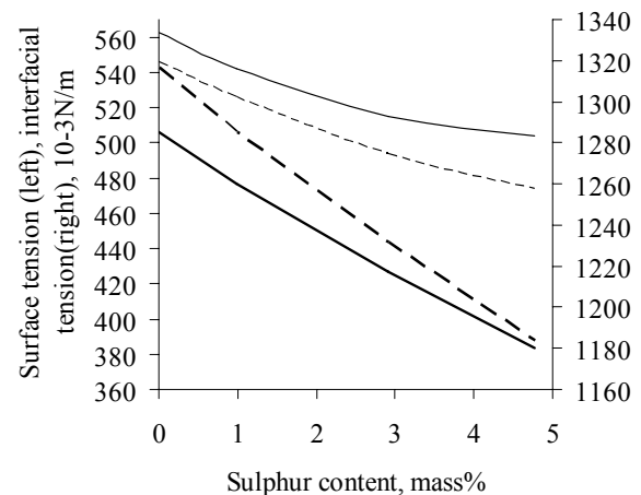
Fig. 2. Influence of the sulphur content in slag \text{CaO-Al}_2\text{O}_3\text{-CaS} at 1873K, on the surface tension of the slag and on the interfacial tension slag-steel. Surface tension (---) C/A=1.5 ; (---) C/A=1 . Interfacial tension (—) C/A=1.5 ; (---) C/A=1 .
