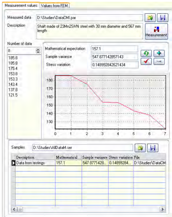
Fig. 6. Data obtained during measurements from testing of reducer shaft (a) and data obtained by the finite-element model (b).
