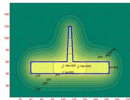
Fig. 8. Distribution of isotherms at the end of solidification for a rib of inclination \text{tg } \alpha = 3/60 and thickness b_n = 5 mm (at the moment of solidification t_{\text{sol}}=193.44\text{s} ).
