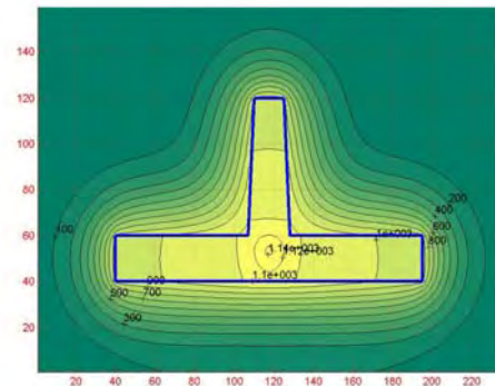
Fig. 12. Distribution of isotherms at the end of solidification for a rib of inclination \text{tg } \alpha = 3/60 and thickness b_n = 15 \text{ mm} (at the moment of solidification t_{\text{sol}} = 407.58\text{s} ).
