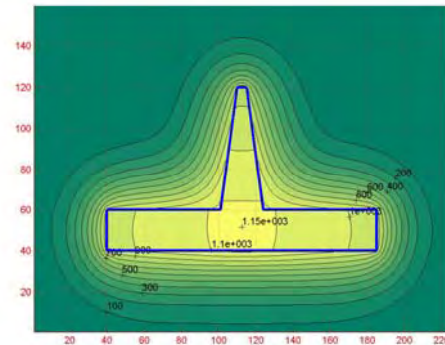
Fig. 10. Distribution of isotherms at the end of solidification for a rib of inclination \text{tg } \alpha = 9/60 and thickness b_n = 5 \text{ mm} (at the moment of solidification t_{\text{sol}} = 366.12\text{s} ).
