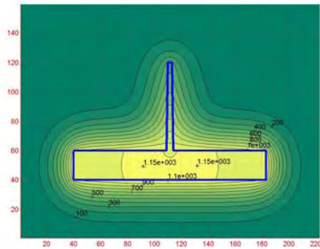
Fig. 3. Distribution of isotherms at the end of solidification for a rib of inclination \text{tg } \alpha = 1/60 and thickness b_n = 3 mm (at the moment of solidification t_{\text{sol}}=264.94\text{s} ).
