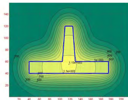
Fig. 13. Distribution of isotherms at the end of solidification for a rib of inclination \text{tg } \alpha = 5/60 and thickness b_n = 15 \text{ mm} (at the moment of solidification t_{\text{sol}} = 435.22\text{s} ).
