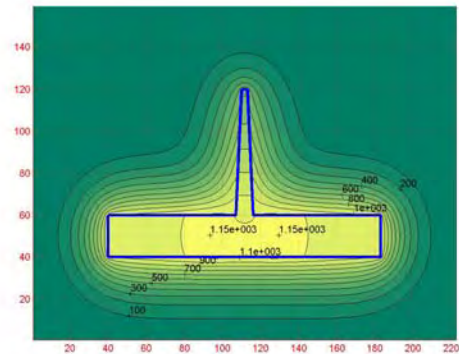
Fig. 4. Distribution of isotherms at the end of solidification for a rib of inclination \text{tg } \alpha = 3/60 and thickness b_n = 3 mm (at the moment of solidification t_{\text{sol}}=277.12\text{s} ).
