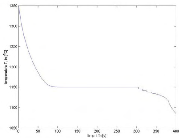
Fig. 17. Temperature variation in the hot spot (coordinates x = 0\text{ mm} , y = 2.5\text{ mm} ), part with a rib of b_n = 15\text{ mm} and inclination \tan \alpha = 1/60 ( T = temperature; t = time).
