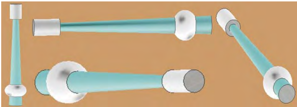
Fig. 5. 3D images obtained for bell tongue with Autodesk Inventor software.
