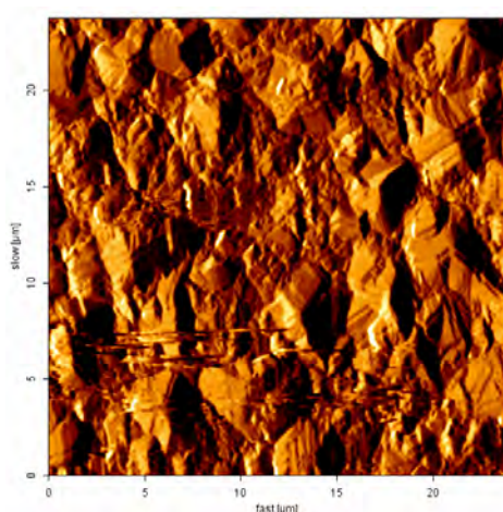
Fig. 6. AFM of SiC/Ni nano composite coating surface 2D – Vertical deflection ( i = 4 A/dm^2 for 1h ): (A) – untreated; (B) – with SRB bacteria.
