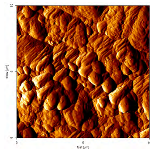
Fig. 5. AFM of nickel surface ( i = 4 A/dm^2 for 1h): A- untreated surface; (B) with SRB, 2D – Vertical deflection.
